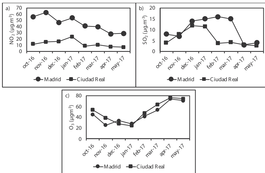
Fig. 1. Air pollution data from Madrid and Ciudad Real during the period of plants development until the pollen collection.
