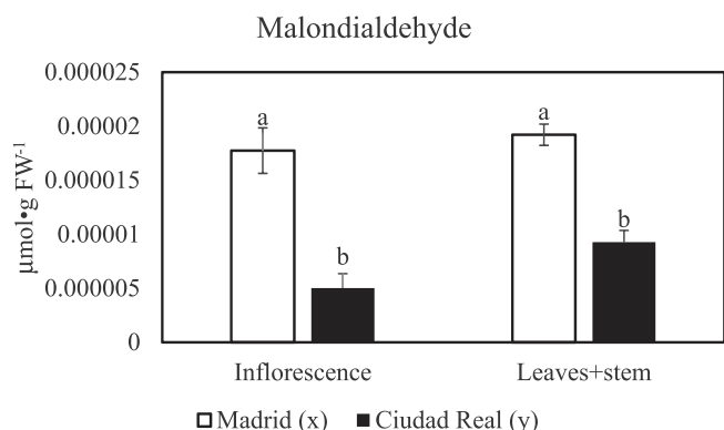
Fig. 5. Concentration of Malondialdehyde (MDA) in plants of Lolium perenne growing in Madrid and Ciudad Real. MDA was measured as \mu\text{mol g FW}^{-1} (fresh weight). Different letters indicate significant differences ( P < 0.05 ) according to LSD.
